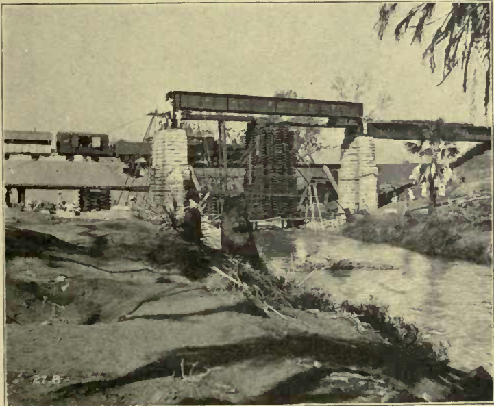
"AND FINALLY LOWERED GENTLY INTO POSITION."
