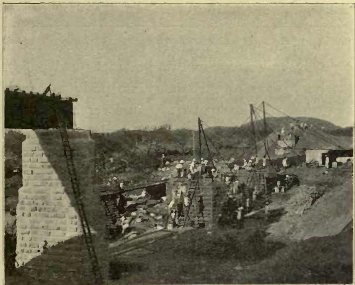
“THE BRIDGE OVER THE TSAVO RAPIDLY NEARED COMPLETION.”
