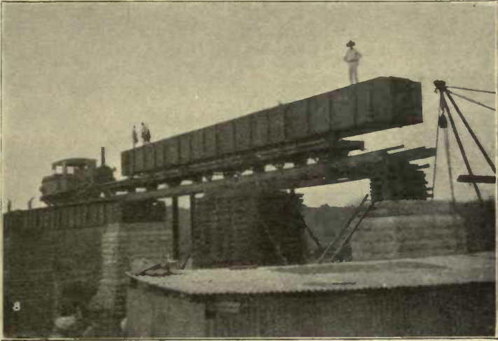
"THE GIRDER WAS RUN OVER ITS EXACT PLACE,"
